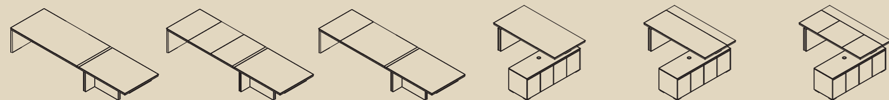
AR 69 3400/1000/750 AR 19 3400/1000/750 AR 29 3400/1000/750 AE 03 2000/1000/750-1250 AE 13 2000/1000/750-1250 AE 23 2000/1000/750-1250 AR 60 3600/1000/750 AR 10 3600/1000/750 AR 20 3600/1000/750 AE 04 2200/1000/750-1250 AE 14 2200/1000/750-1250 AE 24 2200/1000/750-1250
